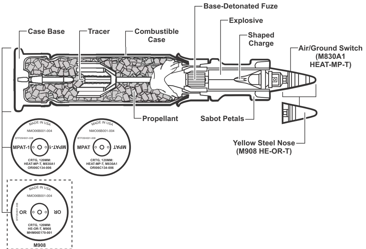
Figure F-4. M830A1 Multipurpose Antitank-Tracer
