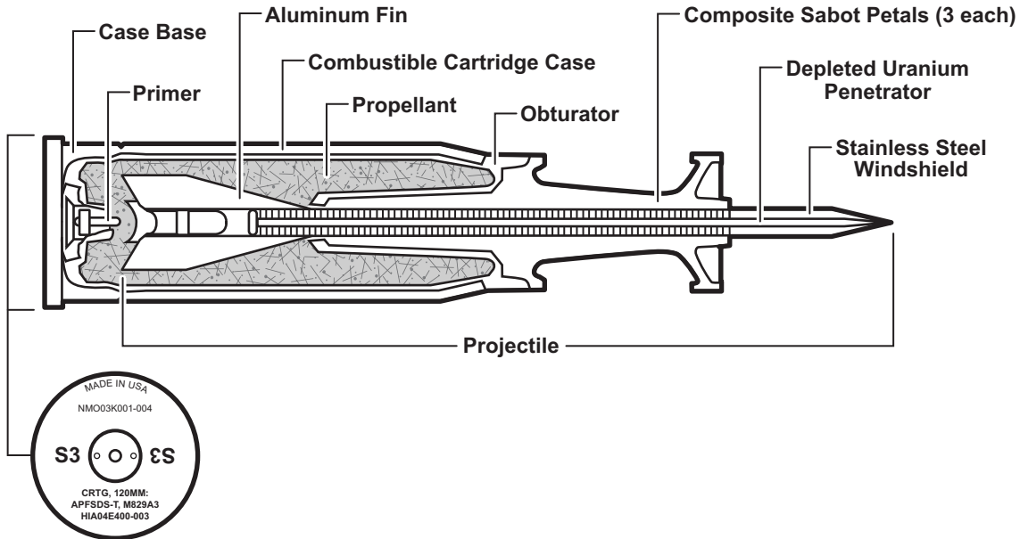
Figure F-1. M829A1/M829A2/M829A3
