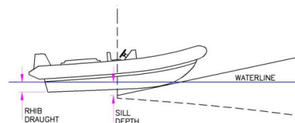
Figure 5 Sill Water Depth
