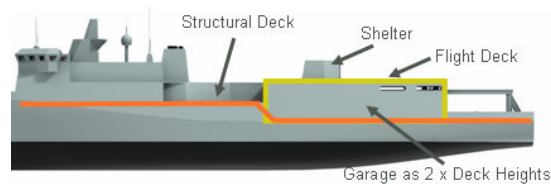
Figure 9 Garage and Flight Deck details
