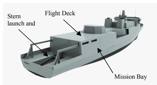
Figure 10 Concept With stern Ramp and Aft Garage
