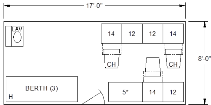
TRIPLE STATEROOM MODULAR GROUP 7 MODIFIED 136 SQ FT GROSS AREA * UNIT 5 MODIFIED TO 36 INCHES WIDE
