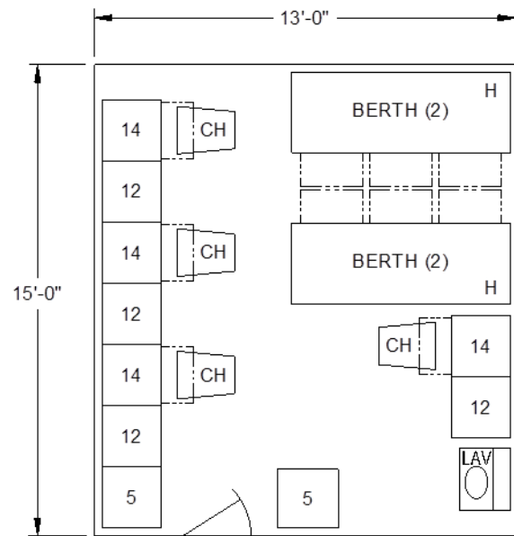
4 PERSON BUNKROOM MODULAR GROUP 7 195 SQ FT GROSS AREA
