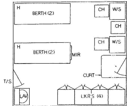
BUNKROOM - 4 CPO OR SNCO
